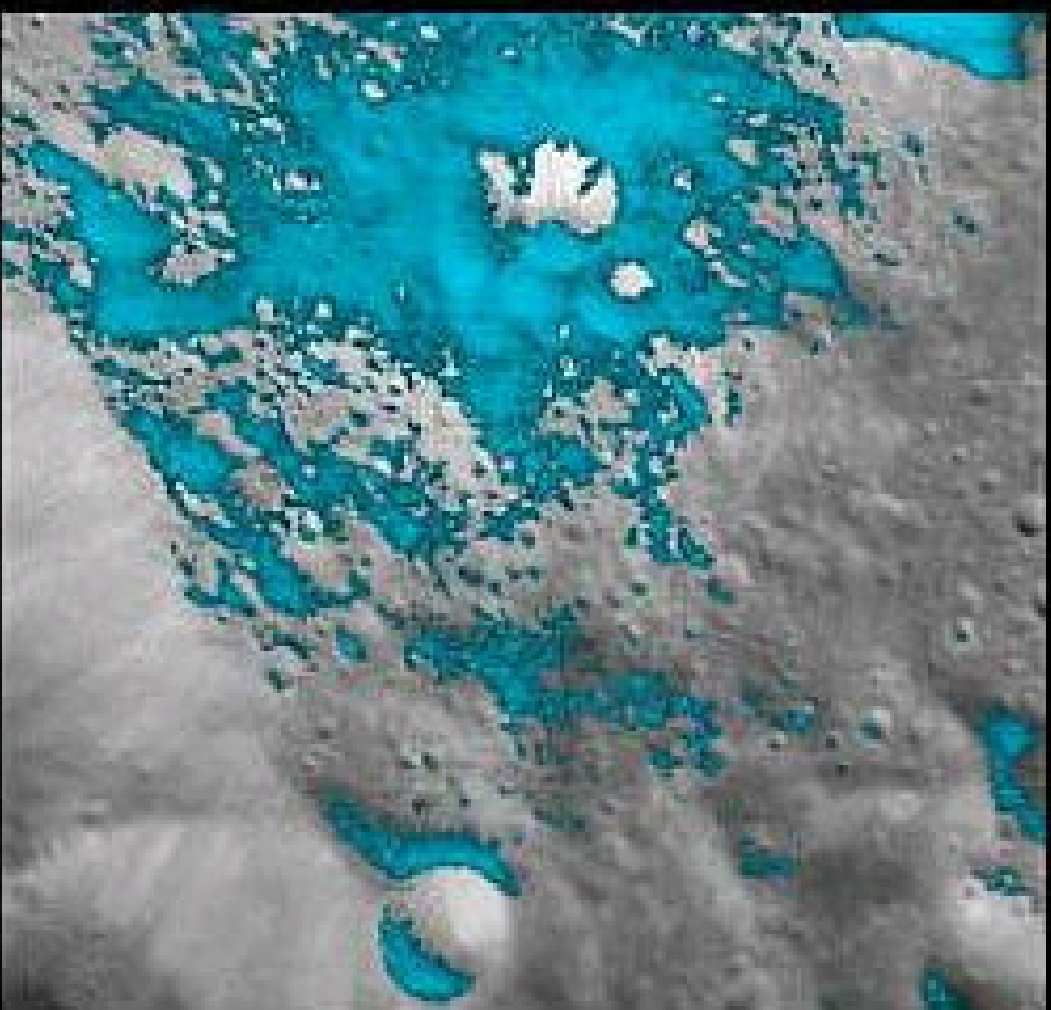
Blue = water absorption strength on Infrared Reflectance
